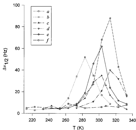
Figure 1. Plot of the line width ( \Delta\nu_{1/2} ) of the ^{31}\text{P} -NMR signal of 4 versus temperature ( T ) in the presence of various resorcinol derivatives (a: [\mathbf{4}]/[\text{octyl 3,5-dihydroxybenzoate}] = 1:6.5 ; b: [\mathbf{4}]/[\text{octyl 3,5-dihydroxybenzoate}] = 1:2 ; c: [\mathbf{4}]/[\text{olivetol}] = 1:7.4 ; d: [\mathbf{4}]/[\text{5-chlororesorcinol}] = 1:6.5 ; e: [\mathbf{4}]/[\text{5-(p-tol)resorcinol}] = 1:4 ; f: 4 without additives) (conditions: solvent \text{CDCl}_3 , [\mathbf{4}] = 8 \times 10^{-3} \text{ M} )
